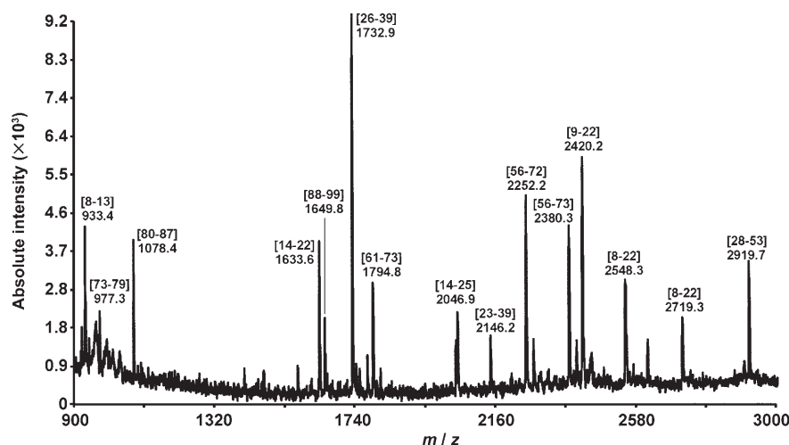
Figure 2. MALDI mass spectrum obtained with the neutral matrix HCCE of peptides (500 fmol) generated by the digestion with endoproteinase Lys-C of cytochrome c labeled with HCCA-NHS. Sequence [14–22], m/z 1634 is the only peak that was also present in the mass spectrum of unmodified cytochrome c .
